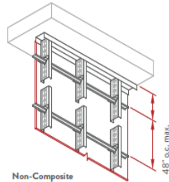
Non-Composite BRACED AT 48" o.c. Gypsum board placed on only one side
